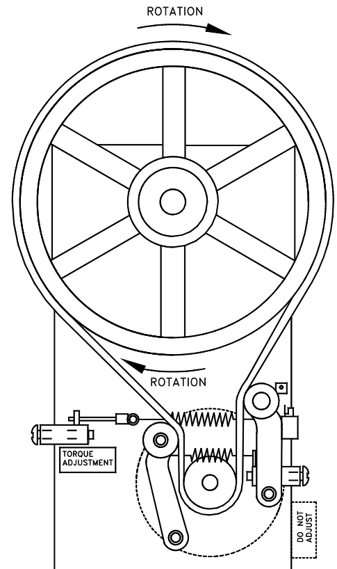
Fig. 39 Mechanical Consistency Control
