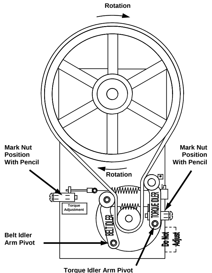
Fig. 44 Spring Adjustment Mechanism
