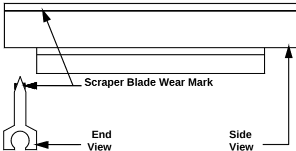
Fig. 41 Scraper Blade Wear Mark
