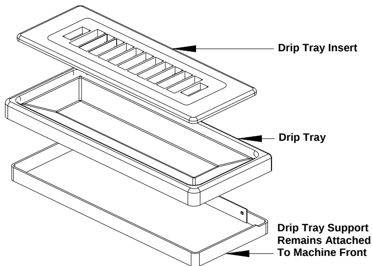
Fig. 20 Drip Tray Assembly
